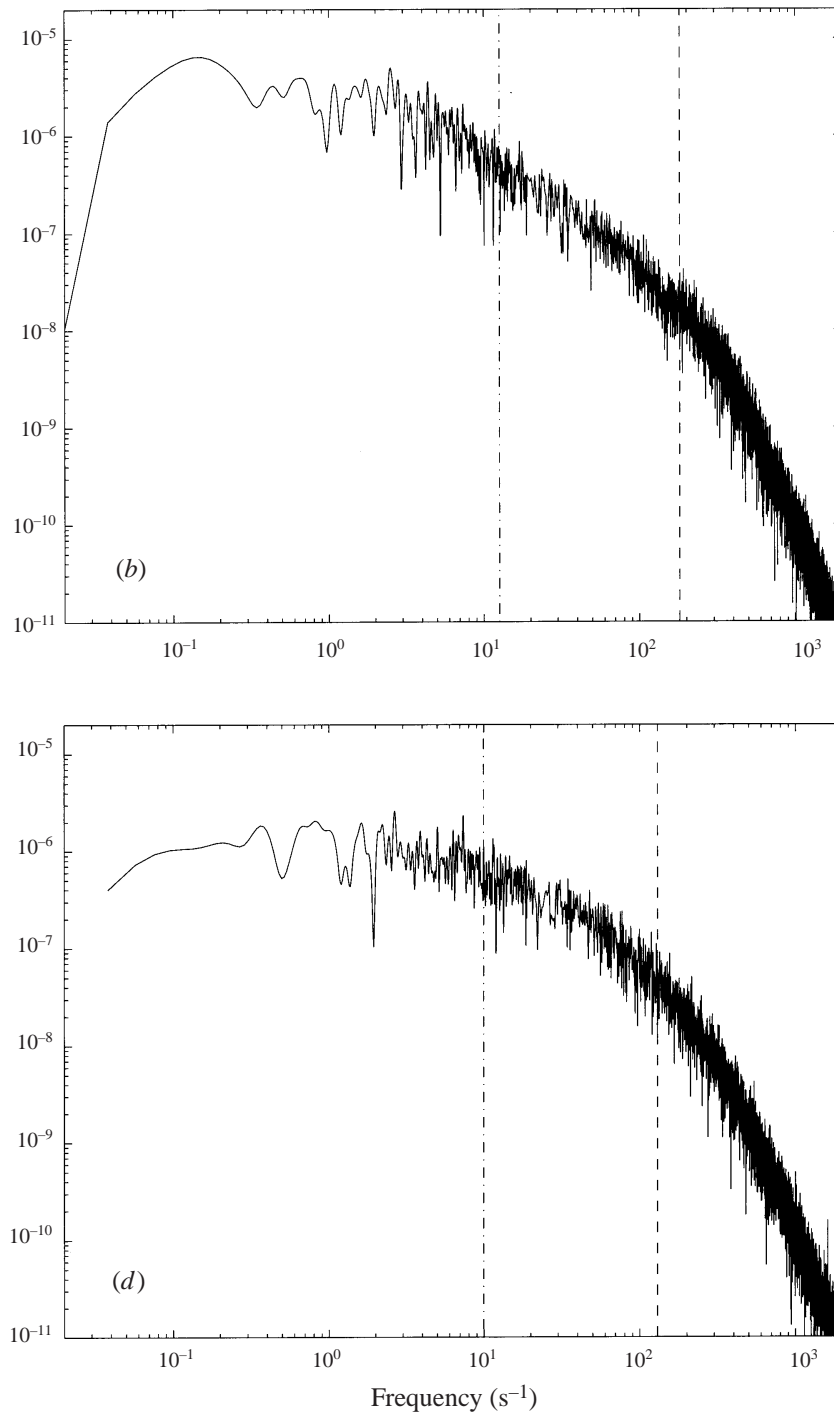
FIGURE 18. Power spectra of the fluid velocity signal for four typical gas volume fractions. The vertical lines denote characteristic frequencies: --- , 2u_b/d_b ; - \cdot - , u_b/H ( H is the gap width). (a) \alpha = 0.01 , (b) \alpha = 0.02 , (c) \alpha = 0.05 , (d) \alpha = 1.10 .
